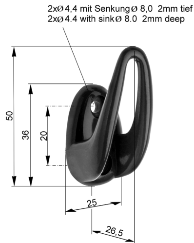
621 0003 dark grey 621 0005 black Coat hook Material: PA 8 g/each
